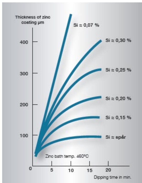
Fig 1. Relationship between dipping time and thickness of zinc coating on steels with different silicon contents. The curves are average curves, based on experiments and practical experience. Significant variations can occur between steels with the same silicon contents, but from different charges.
